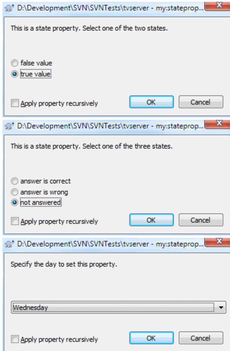
图 4.38. Property dialog state user types
