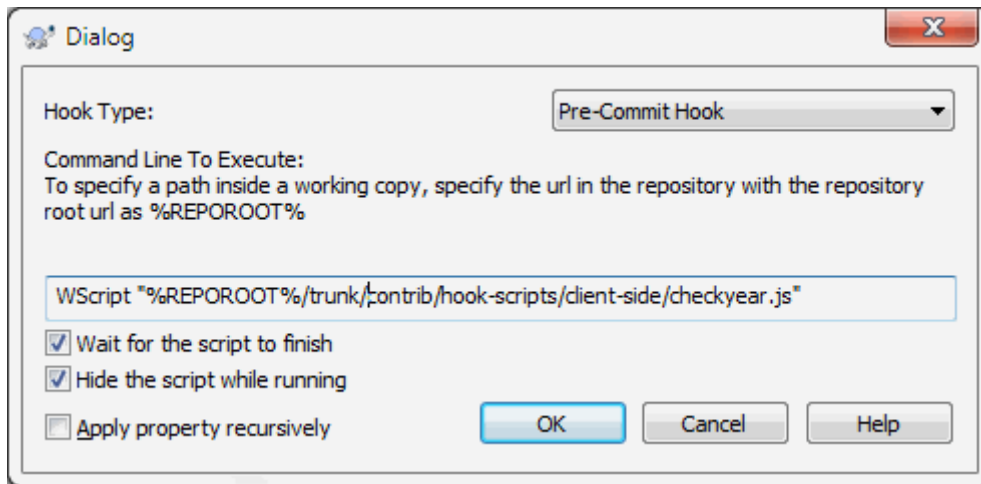
图 4.36. Property dialog for hook scripts
