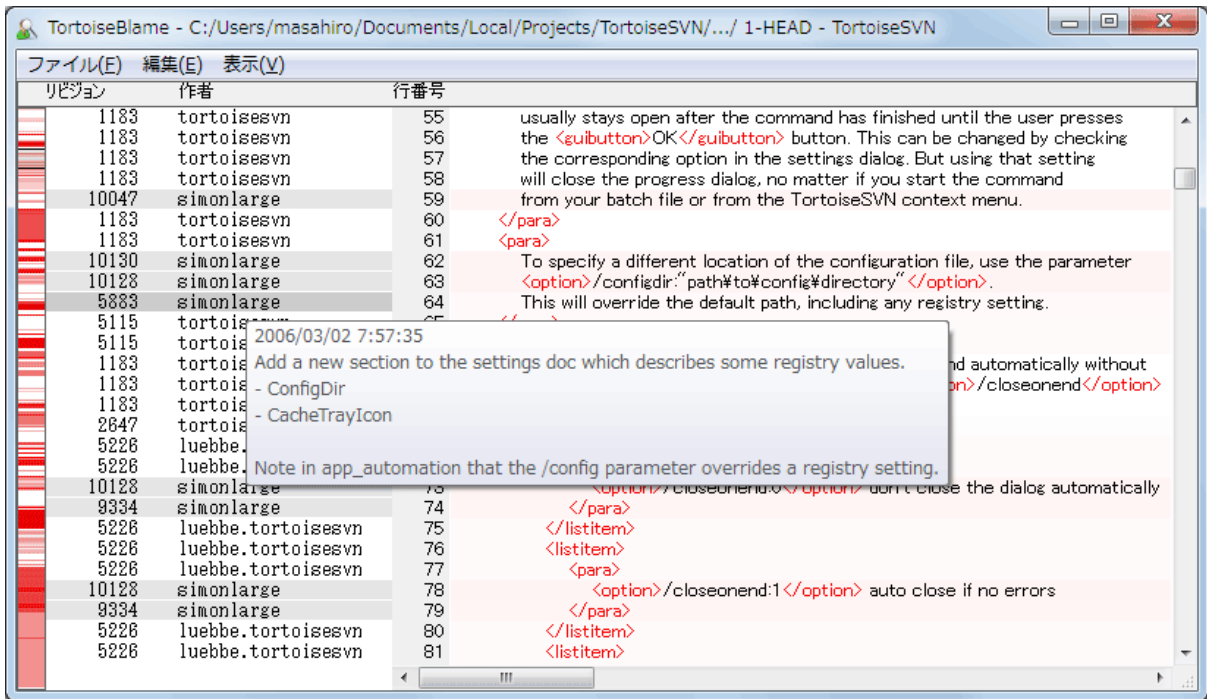
図4.65 TortoiseBlame
