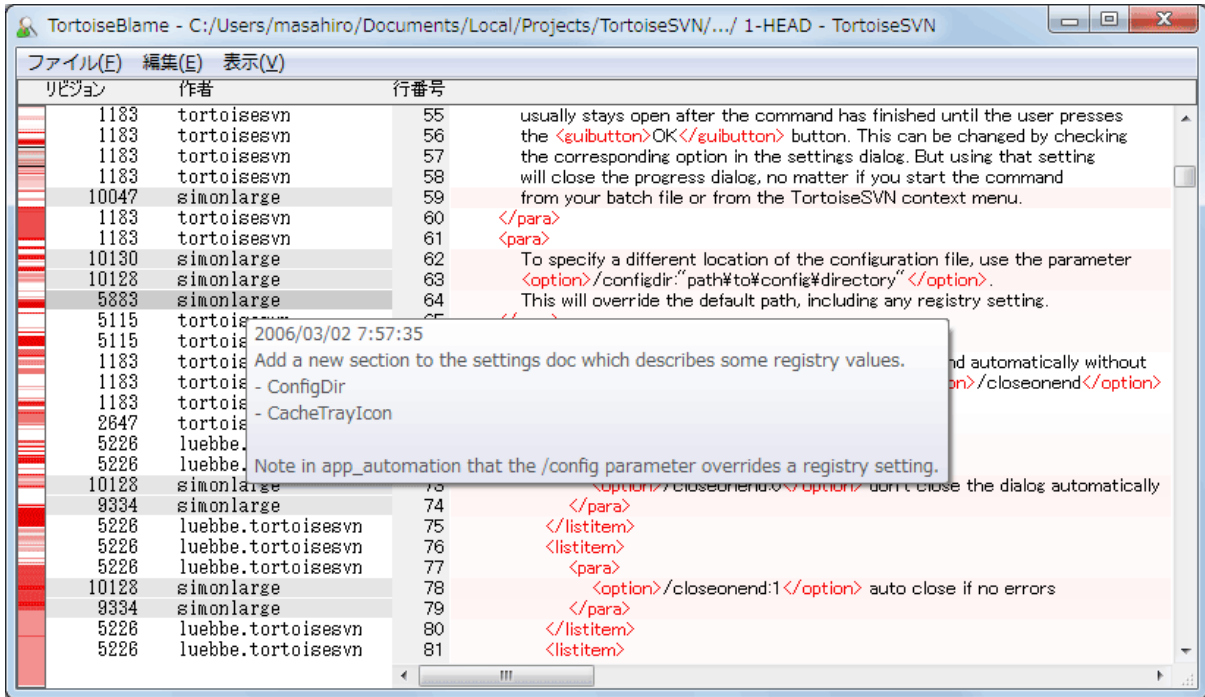
図4.65 TortoiseBlame
