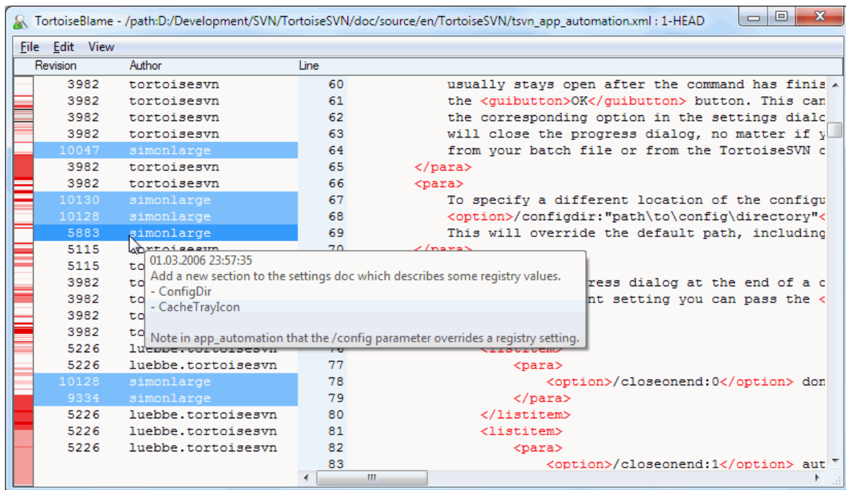
Figure 4.65. TortoiseBlame
