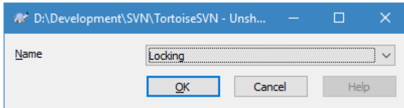
Figure 4.17. Unshelve dialog
