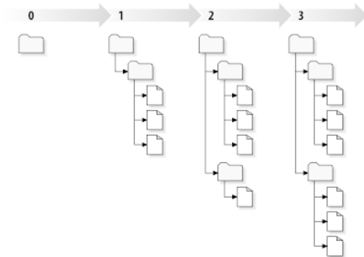
Figure 2.7. The Repository
