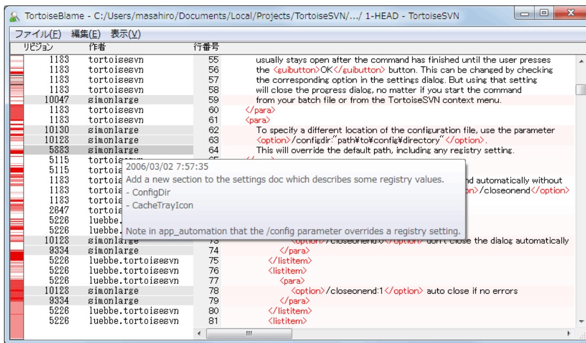
図4.61 TortoiseBlame
