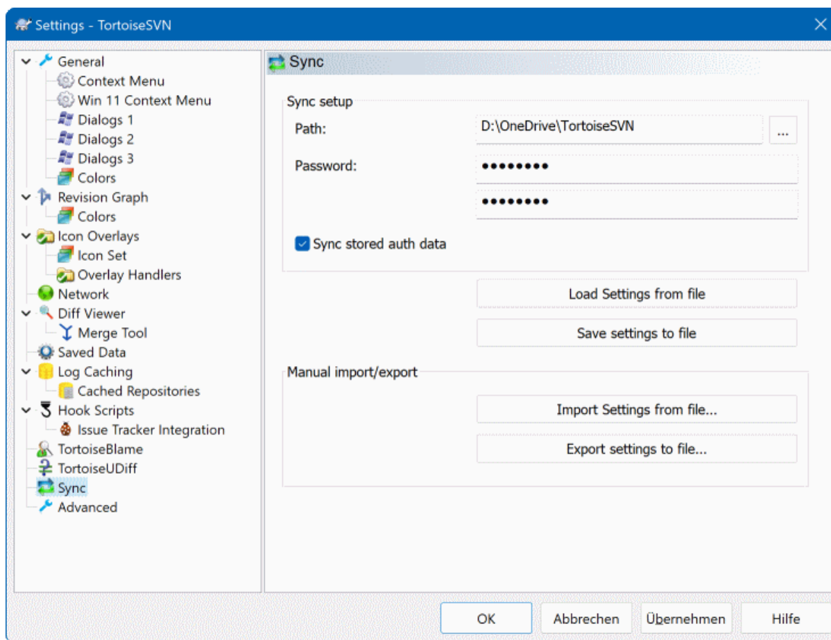
图 4.92. The Settings Dialog, Sync Page
