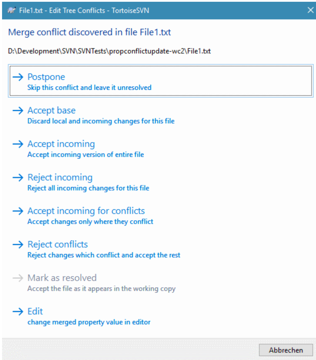
图 4.56. The Merge Conflict Dialog
