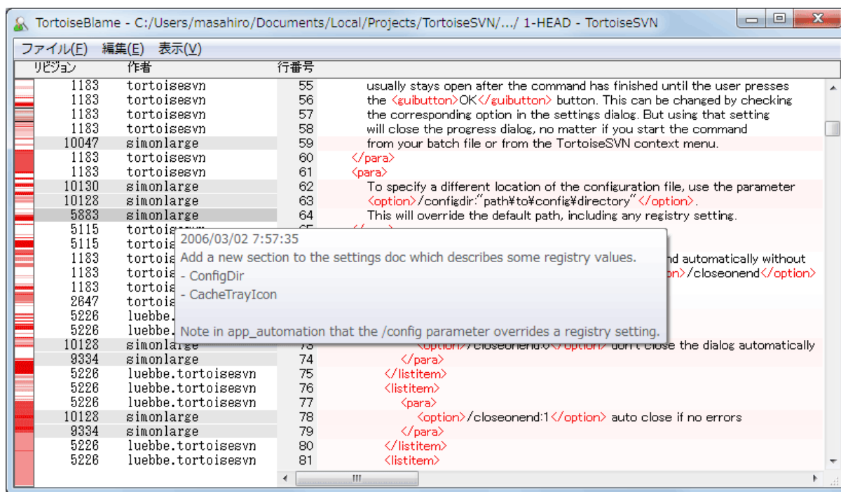
図4.65 TortoiseBlame
