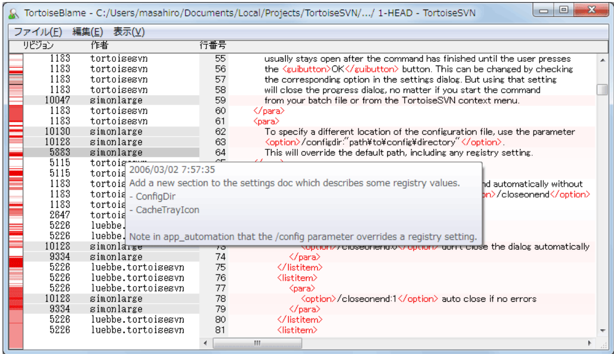
図4.65 TortoiseBlame
