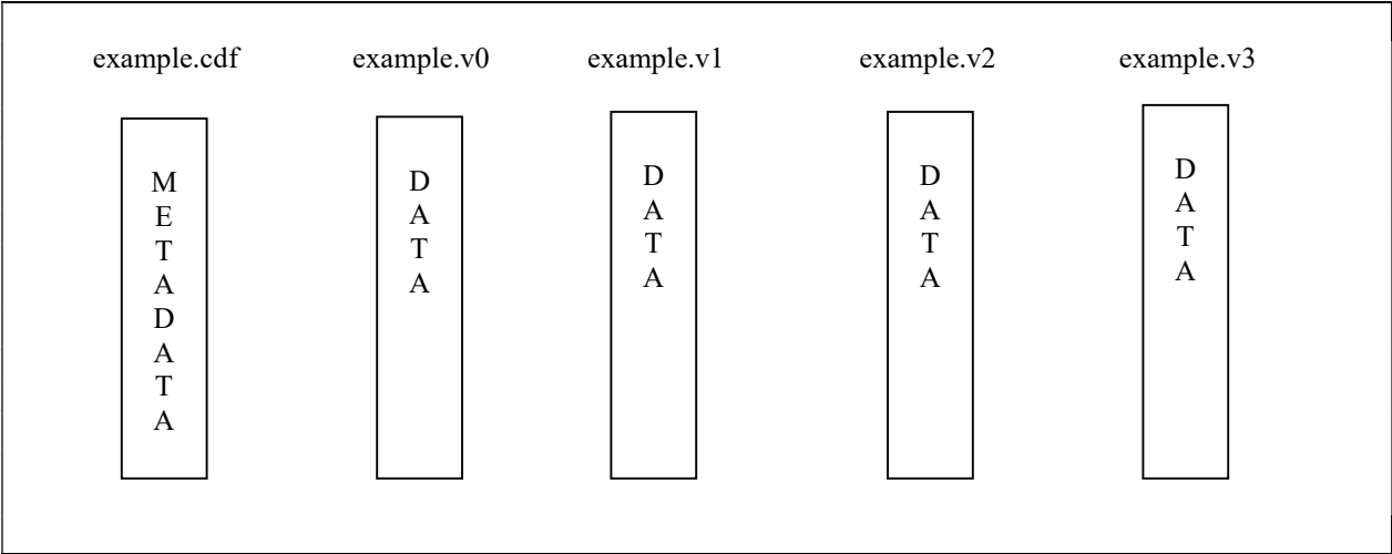
Figure 1.4 Multi-File Format
