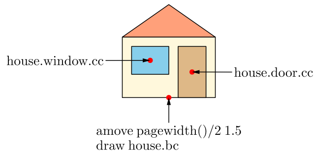
Figure 7.2: Drawing objects and hierarchically named points.
