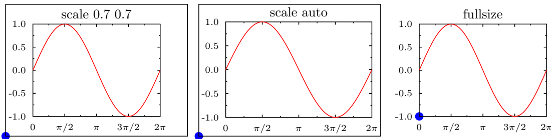
Figure 4.12: Different axis scaling options: default, automatic, and ‘fullsize’. The blue dot indicates the origin (x, y) of the graph, that is, the graph is generated with ‘ move x y ’ followed by ‘ begin graph ’ ... ‘ end graph ’. The xaxis is labeled using the option ‘ format pi ’.
