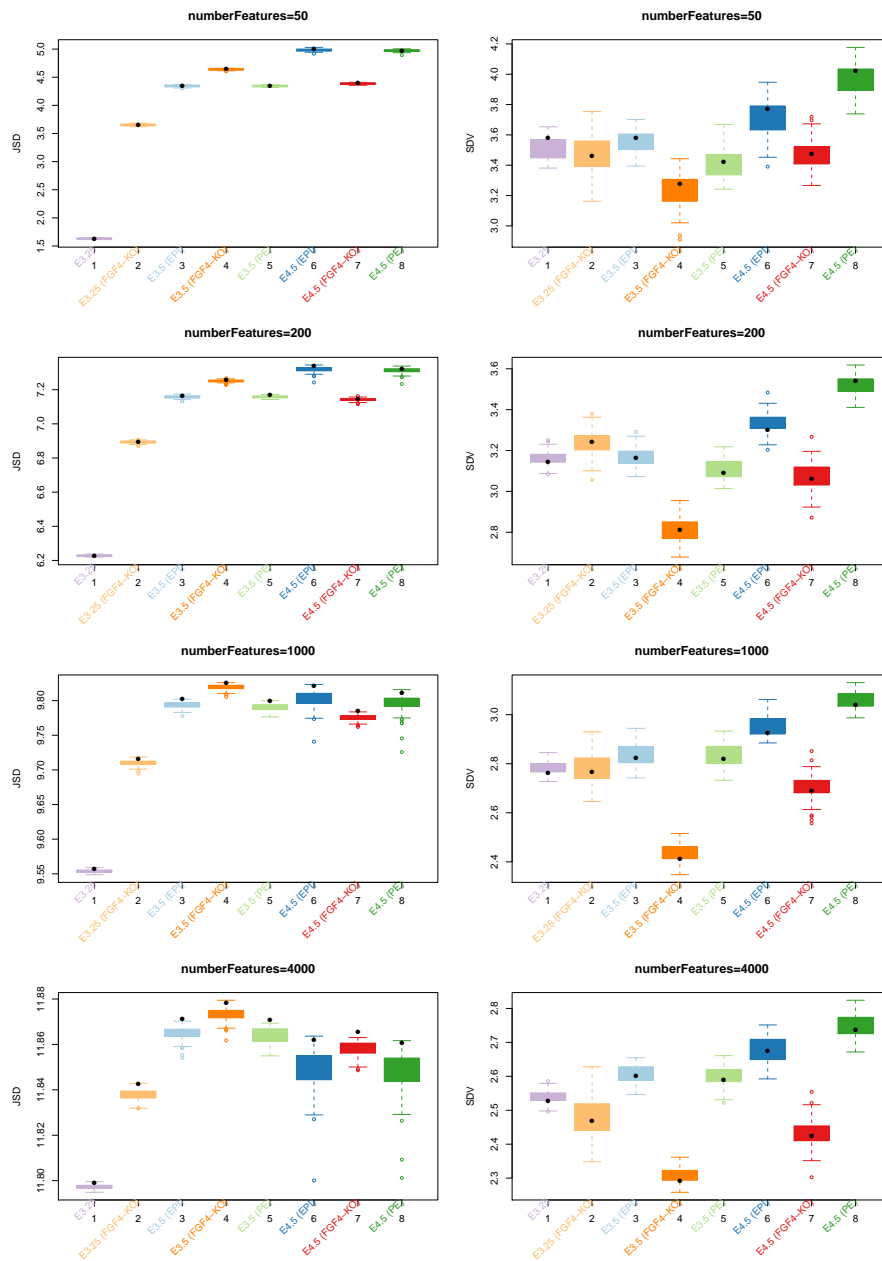
Figure 35: Jensen-Shannon divergences
