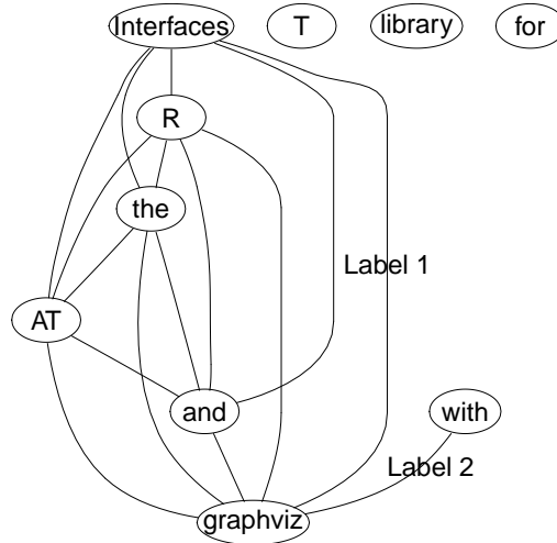
Figure 6: g1 laid out with user-defined node and edge labels.
