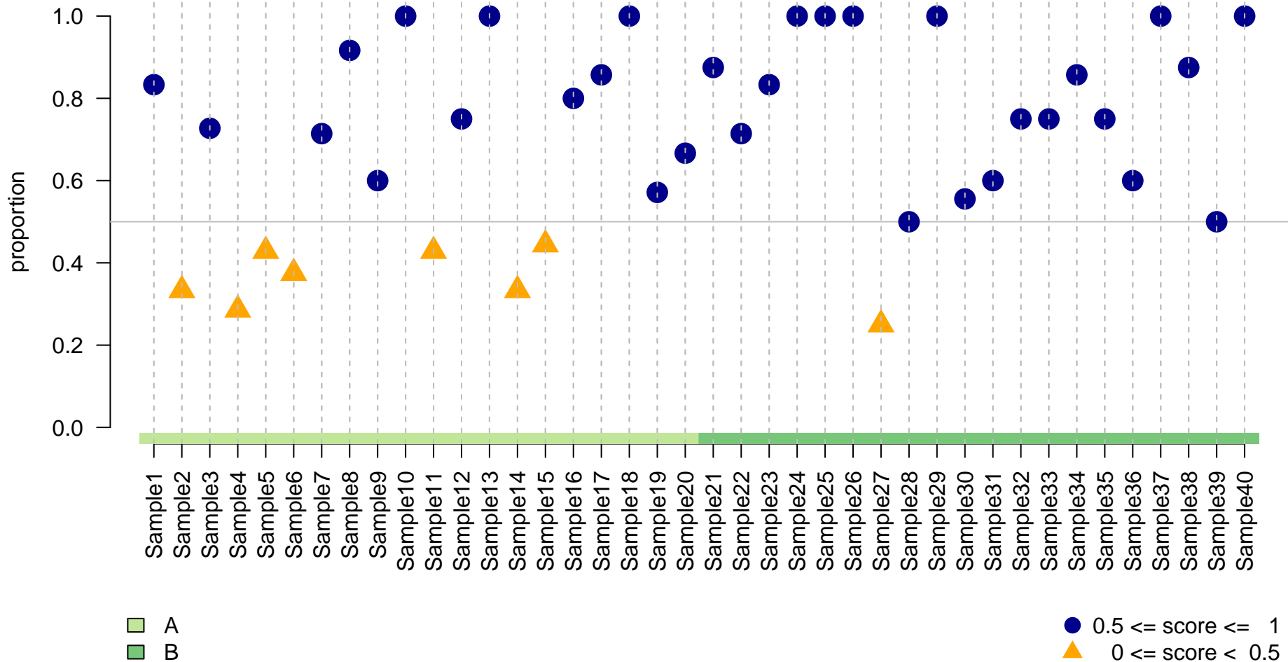
Freq. of being correctly classified (randomForest, 5 feat.)
