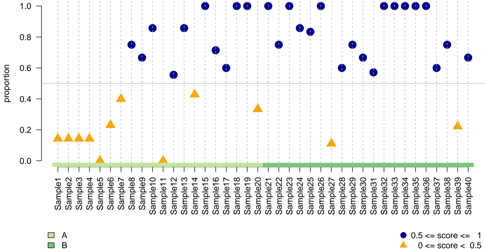
Freq. of being correctly classified (pam, 10 feat.)
