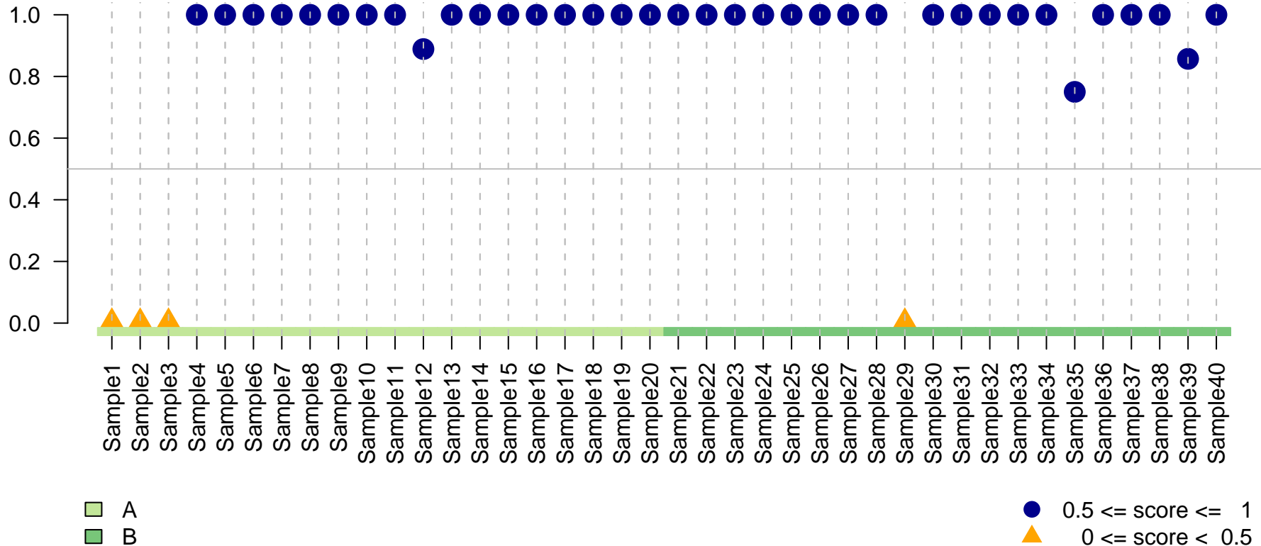
Scores Plot (svm, 5 features)
