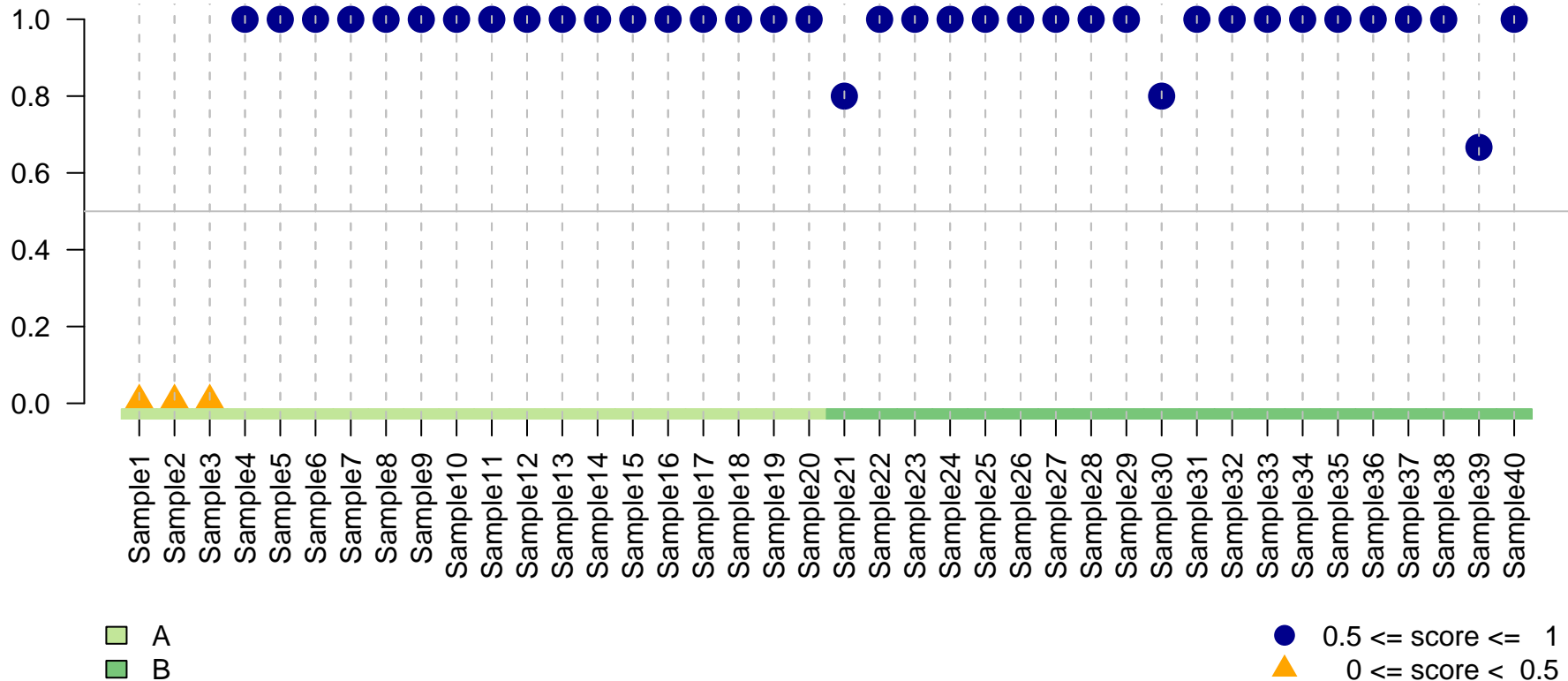
Scores Plot (rf, 7 features)
