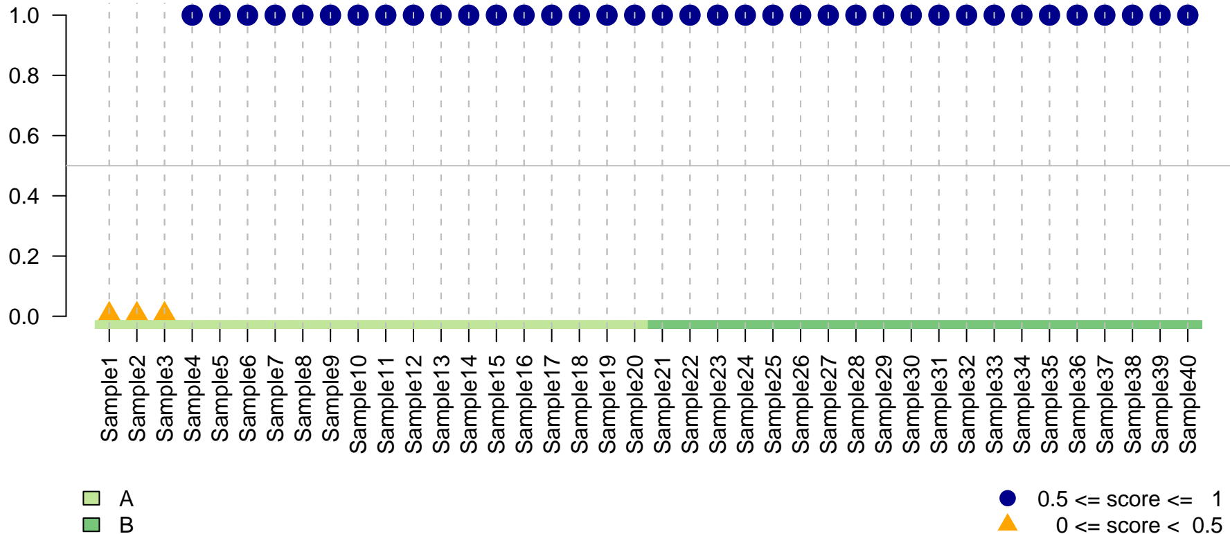
Scores Plot (dlda, 15 features)
