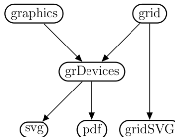
Figure 34: gridSVG [5]
