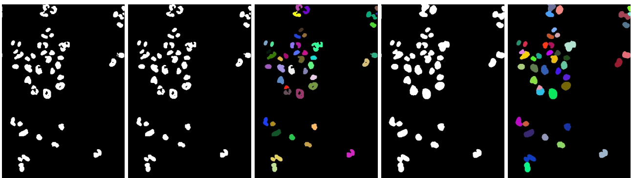
nucleusThresh
