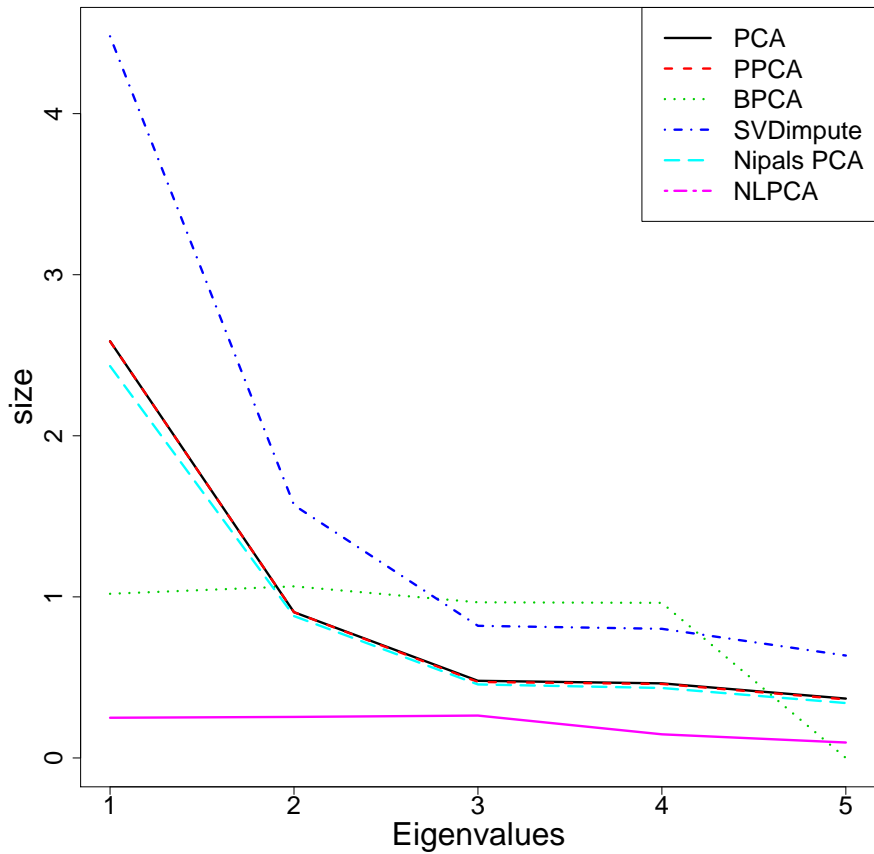
Figure 2: Eigenvalue structure as obtained with different methods
