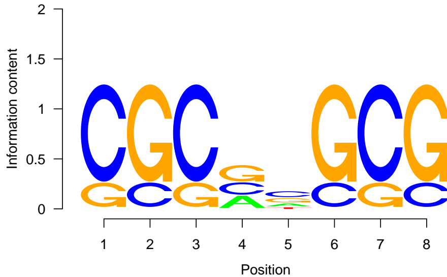
Figure 1: Sequence logo of motif used for simulating sequences.
