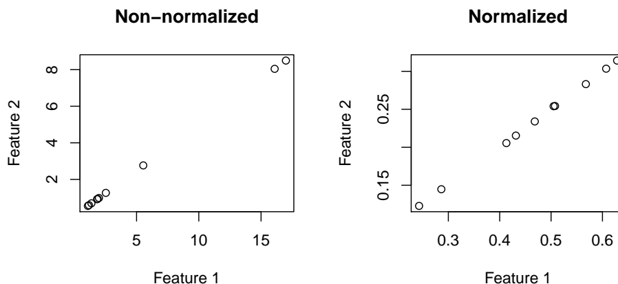
Figure 1: Non-normalized and normalized associations between feature 1 and feature 2 In this case we would expect feature 1 and feature 2 to be associated. In the output we see this by the positive sim.score value in the [1,2] element of test.output$sim.score and the small q -value in the [1,2] element of test.output$q.values .
