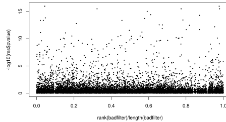
Figure 2: Scatterplot analogous to Figure 1, but with badfilter
