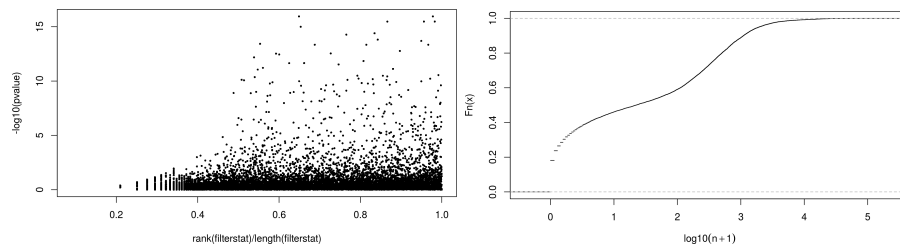
Figure 1: Left: scatterplot of the rank (scaled to [0, 1] ) of the filter criterion filterstat ( x -axis) versus the negative logarithm of the test p value ( y -axis)
