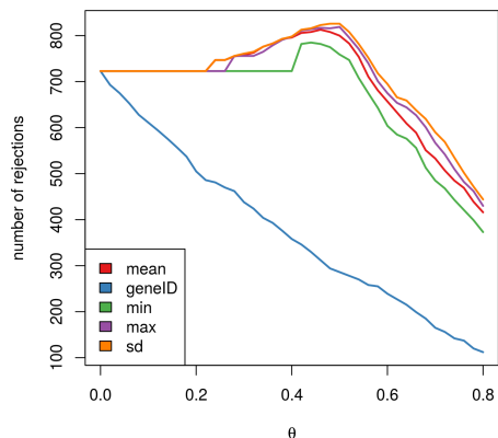
Figure 4: The number of rejections at FDR=10% as a function of \theta (analogous to the right panel in Figure 3) for a number of different choices of the filter statistic
