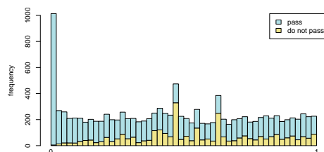
Figure 5: Histogram of p -values for all tests
