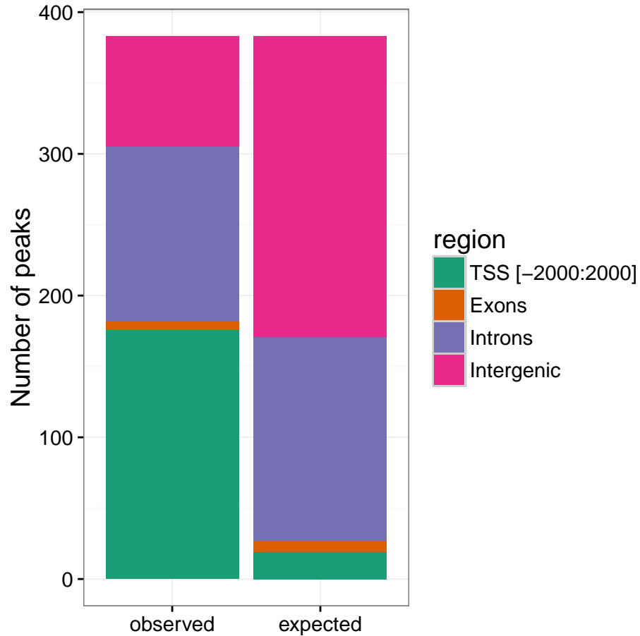
Figure 6: Genomic distribution of the peaks
