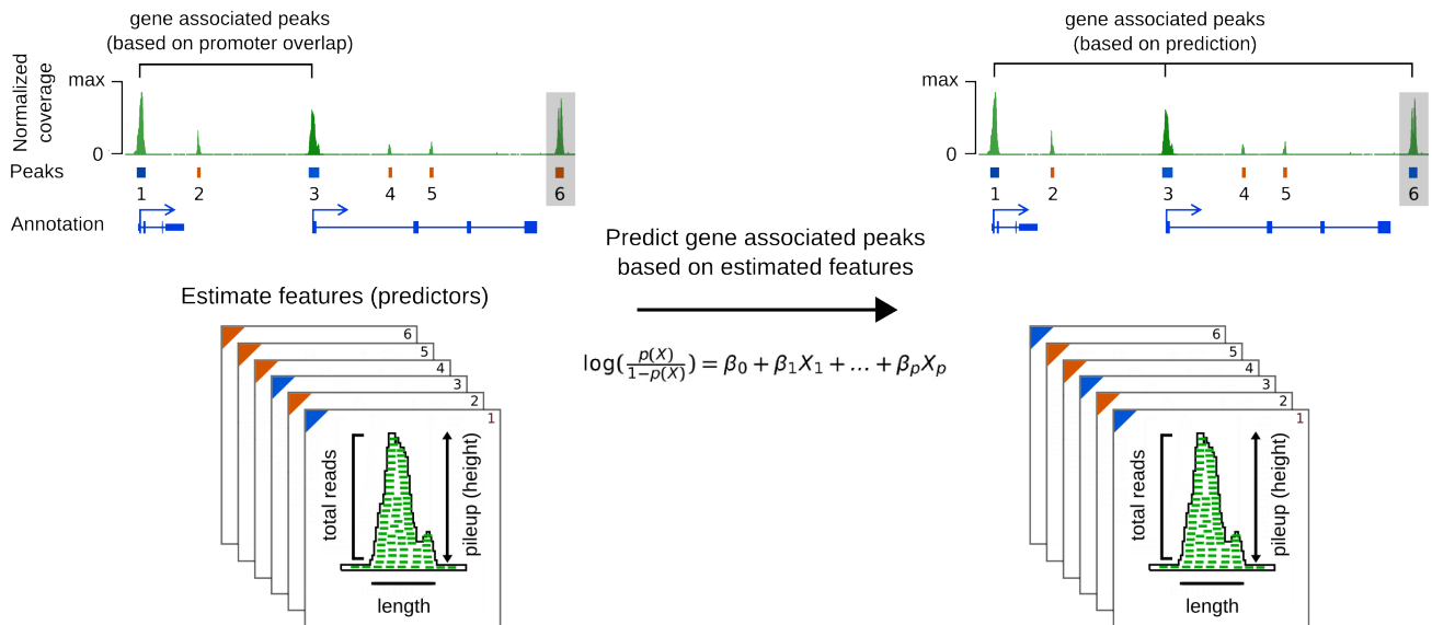
Figure 3: Classification of the peaks on gene associated and background.
