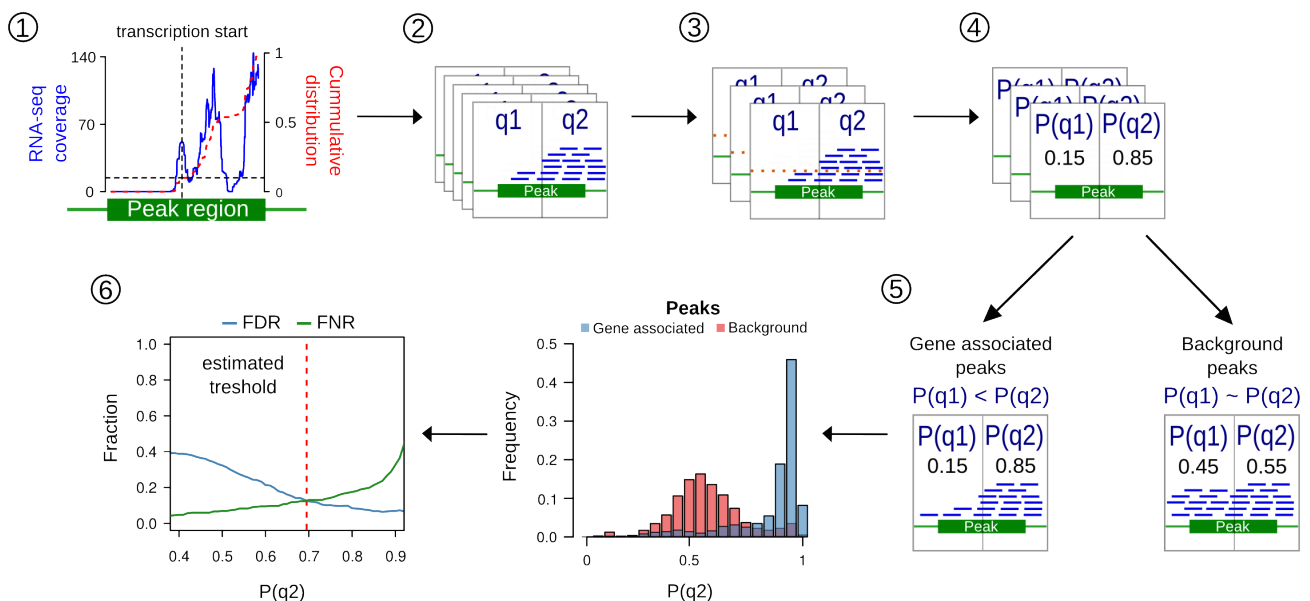
Figure 5: ChIP peak “strandedness” prediction.
