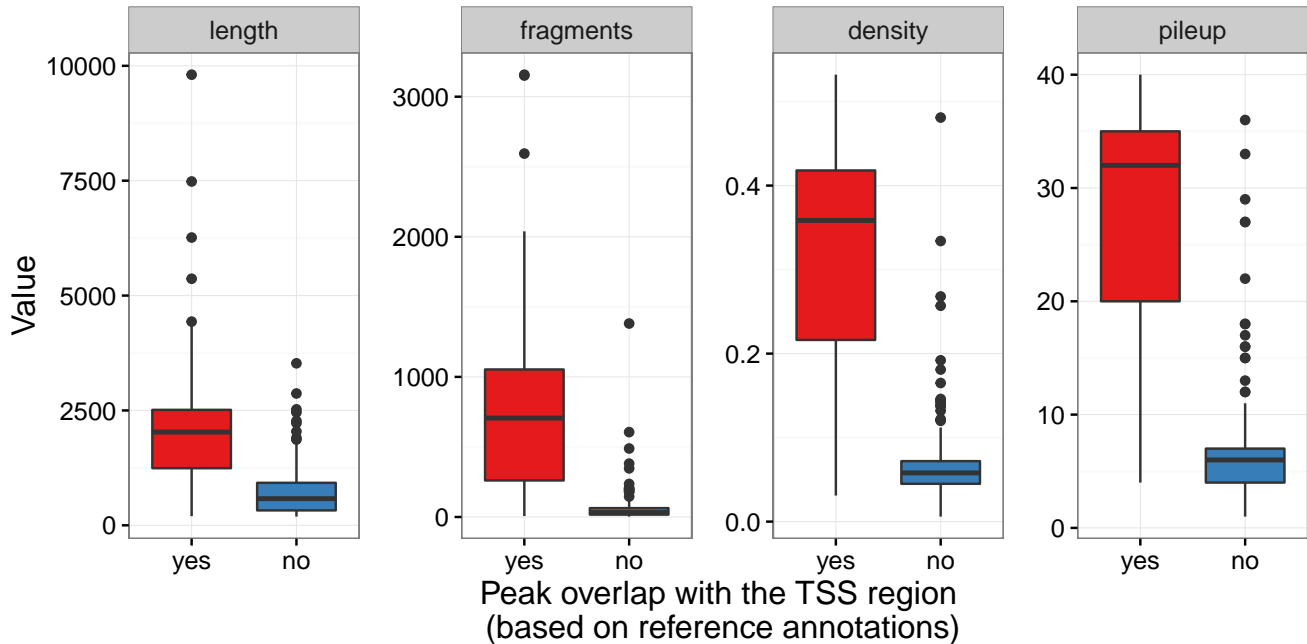
Figure 8: Estimated features
