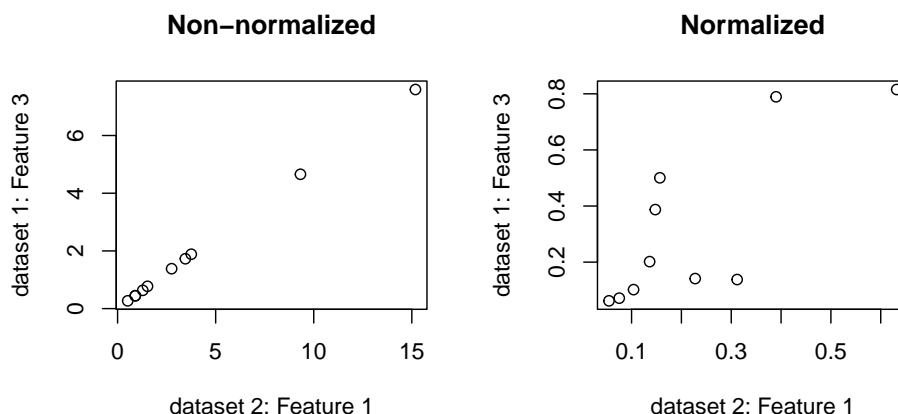
Figure 2: Non-normalized and normalized associations between feature 1 and feature 2
